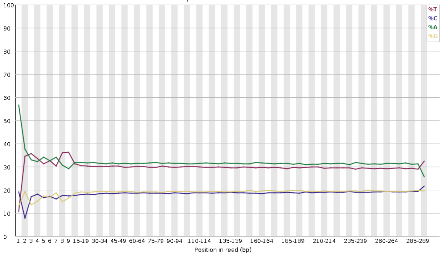
Sequence content across all bases
