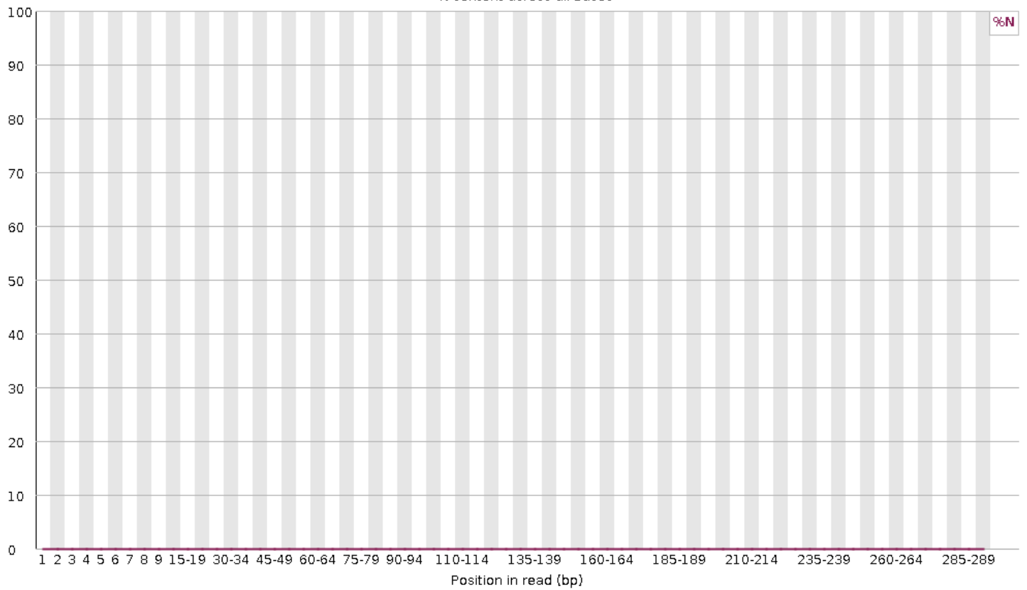
N content across all bases
